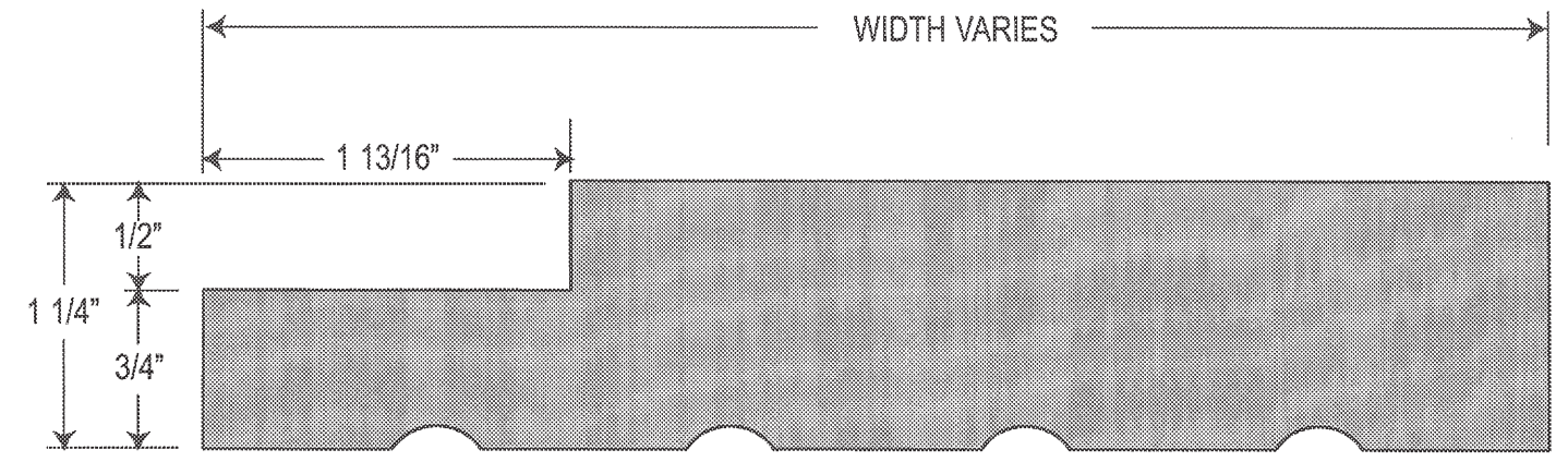
TYPICAL INTERIOR RABBETED JAMB
