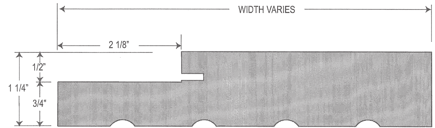
TYPICAL EXTERIOR DOOR JAMBS
